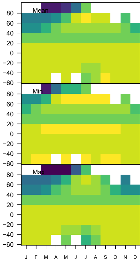
(a) ALBS Model Ensemble (N = 9 )
