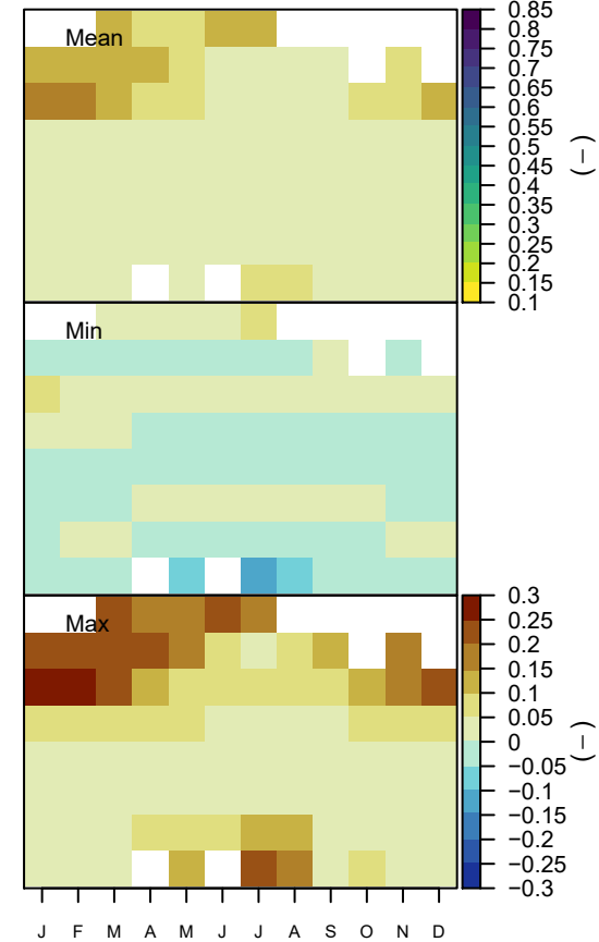
(c) ALBS Mean Ensemble Bias (N = 27 )
