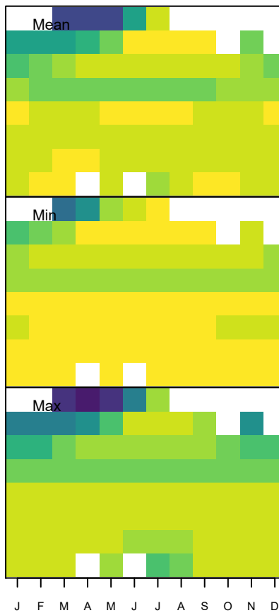
(b) ALBS Reference Ensemble (N = 3 )
