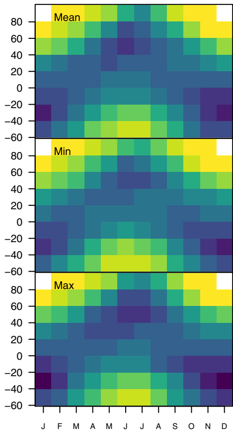
(a) RSS Model Ensemble (N = 6)
