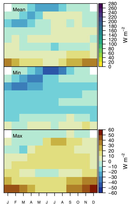
(c) RSS Mean Ensemble Bias (N = 12)
