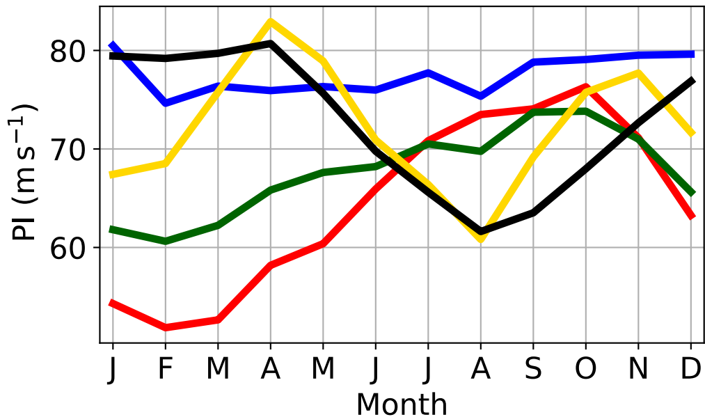
(a) Seasonal Mean Maximum Potential Intensity ( \text{m s}^{-1} )
