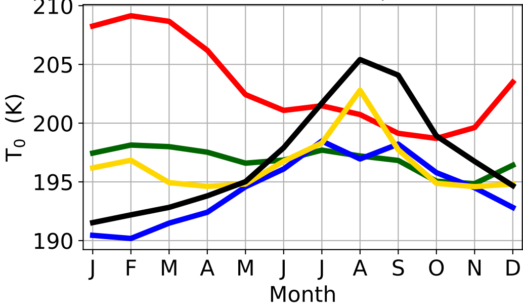
(c) Seasonal Mean Outflow Temperature ( \text{K} )
