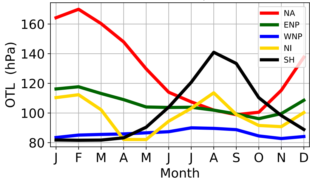
(d) Seasonal Mean Outflow Temperature Level (hPa)
