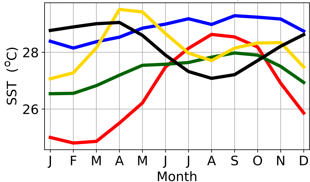
(b) Seasonal Mean Sea Surface Temperature ( ^{\circ}\text{C} )
