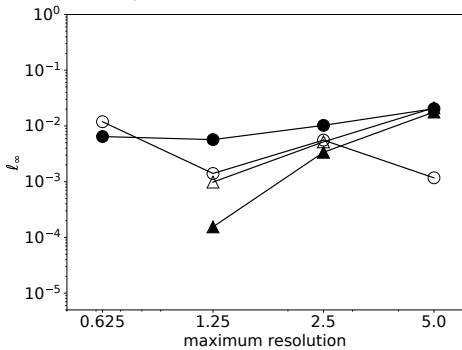
l_\infty error, Courant number around 1
