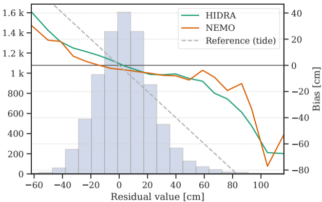
(a) Bias w.r.t. residual
