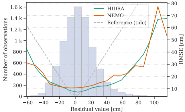
(b) RMSE w.r.t. residual
