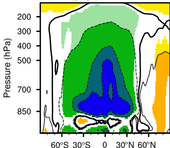
(g) \Delta RH (unitless)
