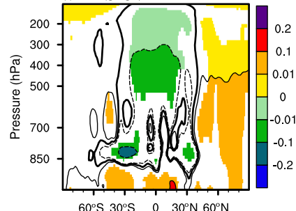
(i) \Delta RH (unitless)
