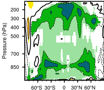
(j) \Delta f (fraction)
