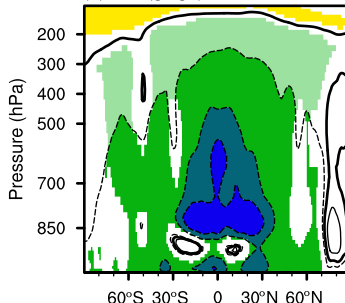
(h) \Delta RH (unitless)
