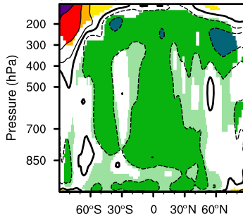
(k) \Delta f (fraction)
