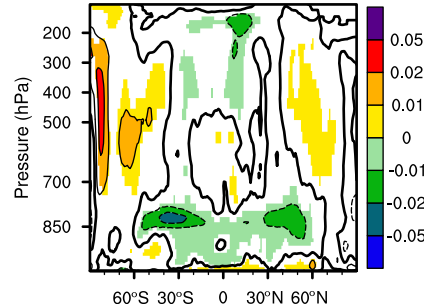
(l) \Delta f (fraction)
