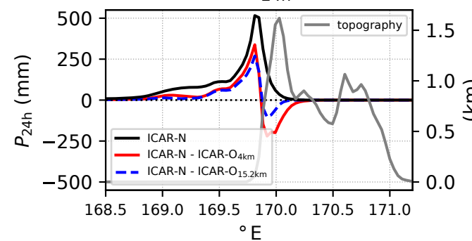
(i) P_{24h}
