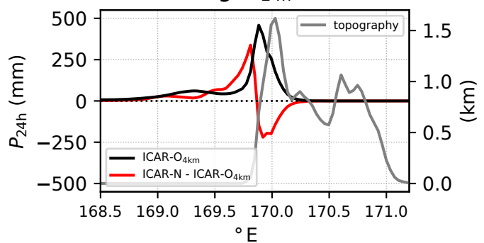
(g) P_{24h}
