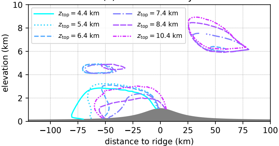
(a) cloud boundary
