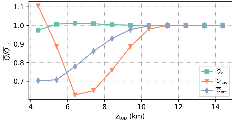
(b) relative total masses of MP species
