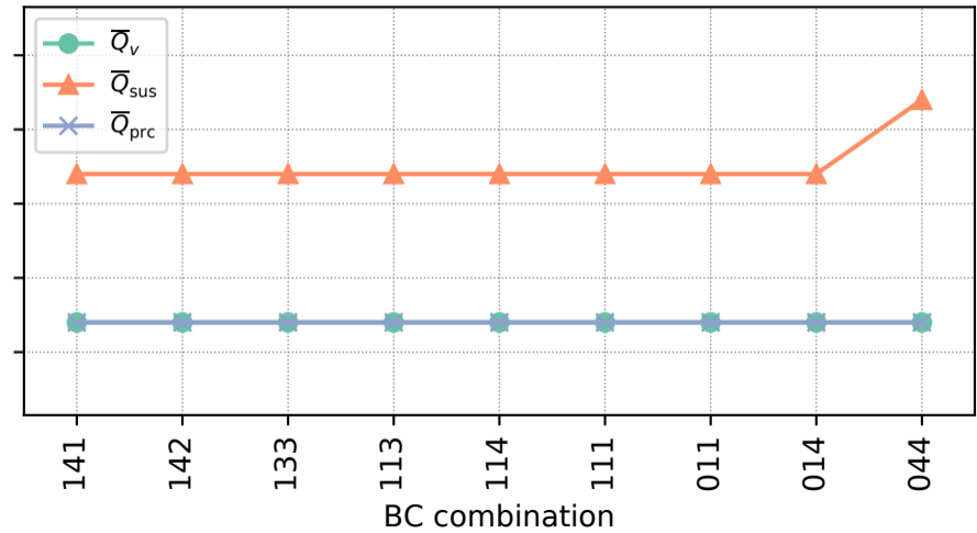
(b) absolute masses
