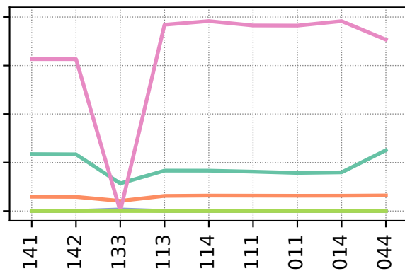
(e) P_{12\text{h}}
