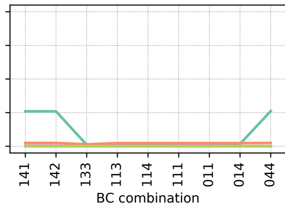
(c) \bar{q}_{\text{sus}}
