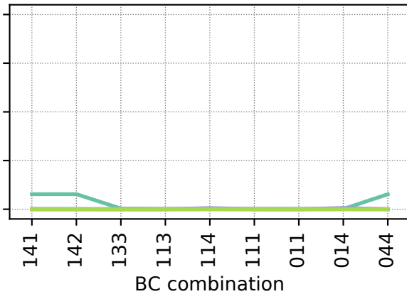
(e) P_{12\text{h}}
