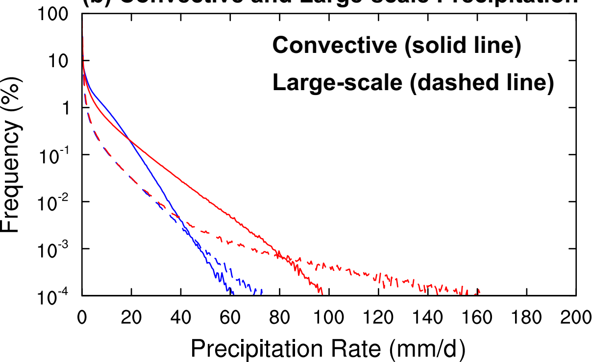
(b) Convective and Large-scale Precipitation
