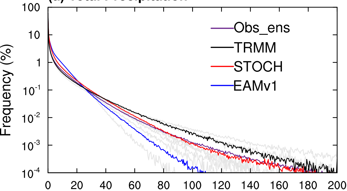
(a) Total Precipitation
