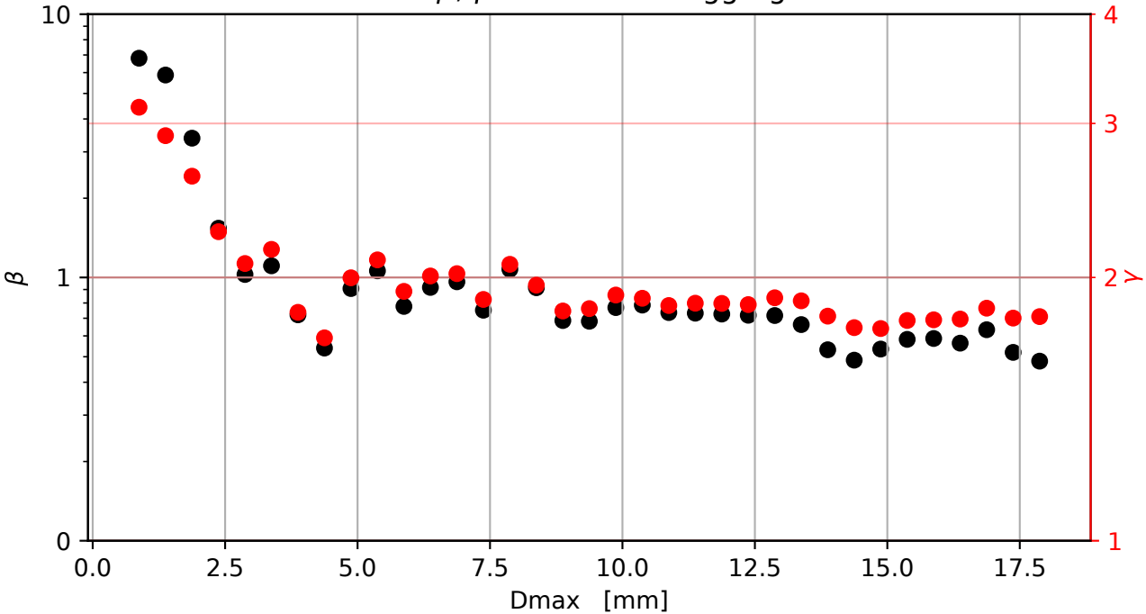
SSRGA \beta, \gamma for dendrite aggregates
