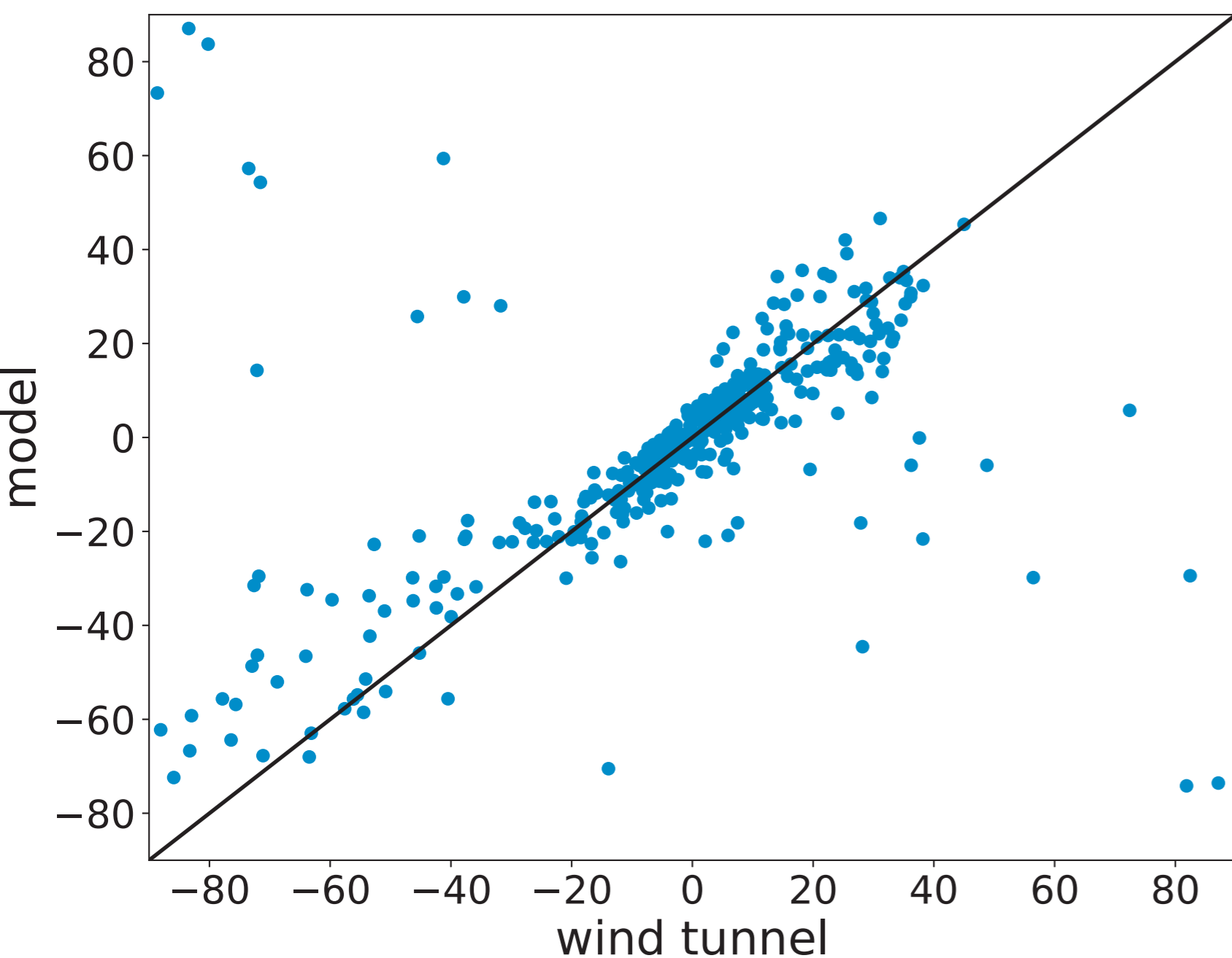
(c) Horizontal wind direction \arctan(v/u) 18 m [°]
