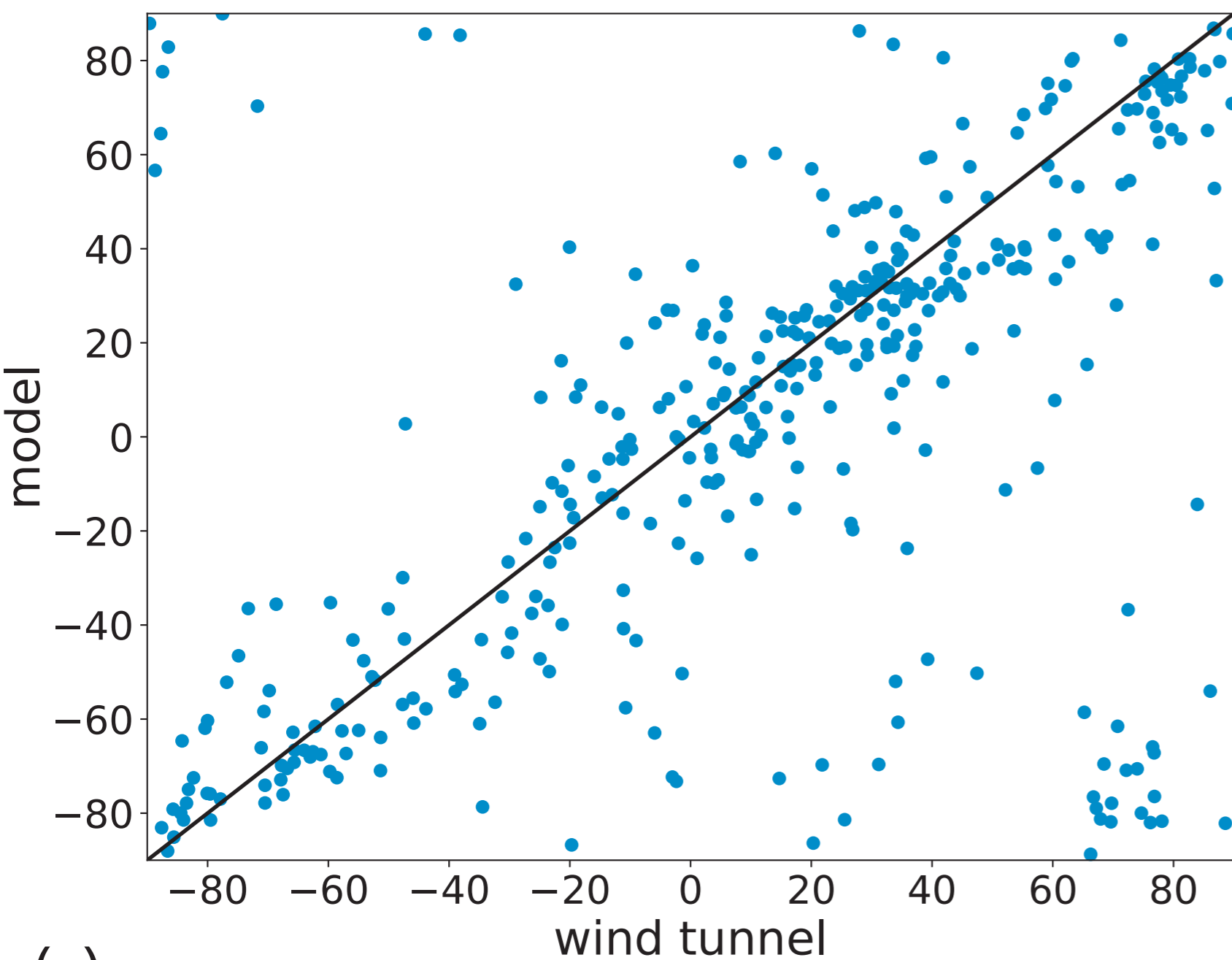
(a) Horizontal wind direction \arctan(v/u) 2 m [°]
