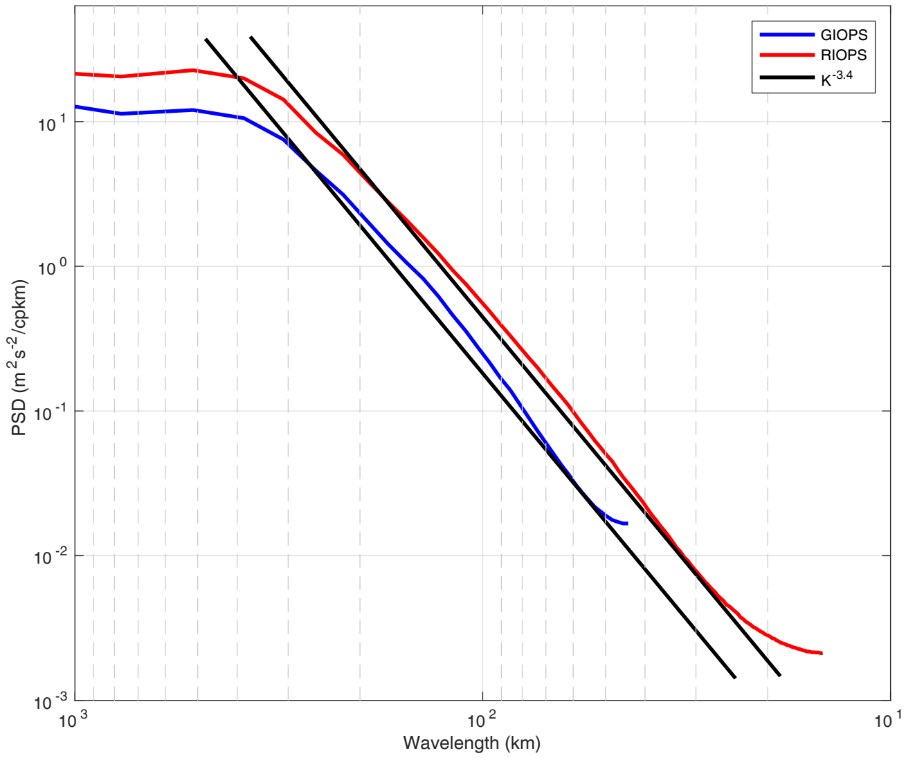
PSD of Surface Kinetic Energy
