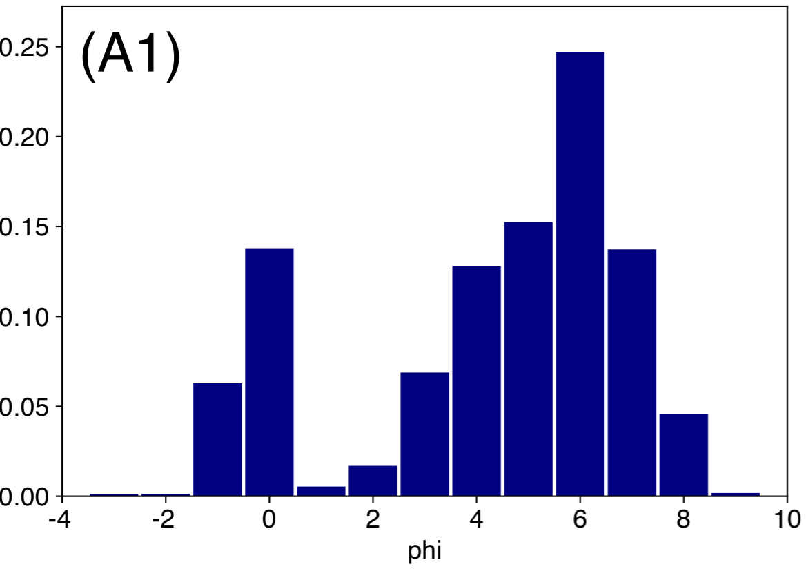
Plume GSD
