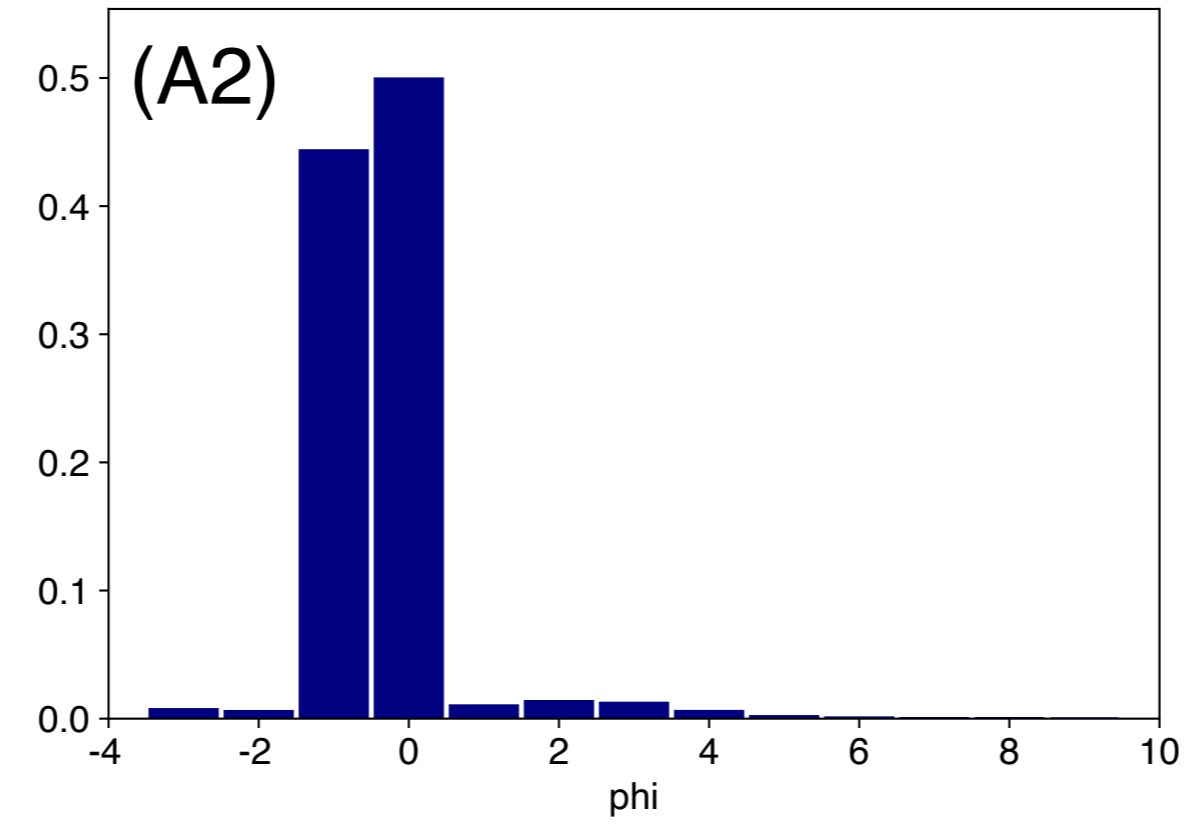
Sedimentation GSD
