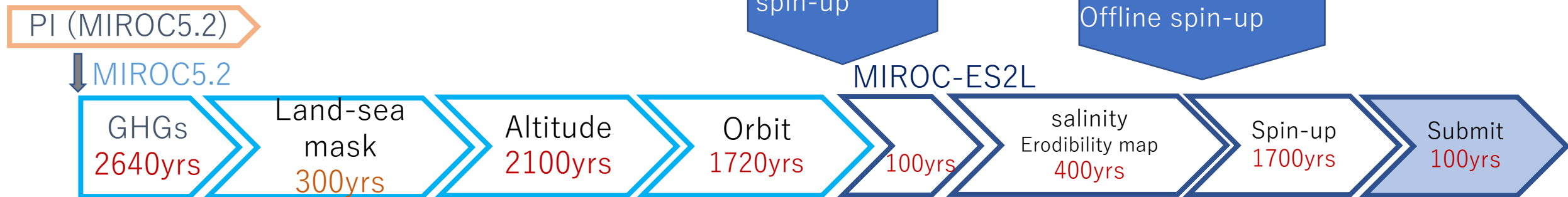
(b) spin-up procedure of 6ka
