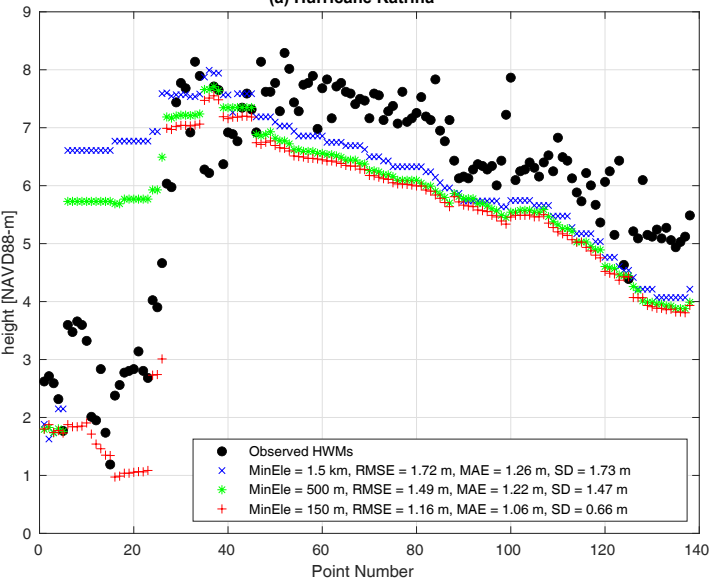
(a) Hurricane Katrina
