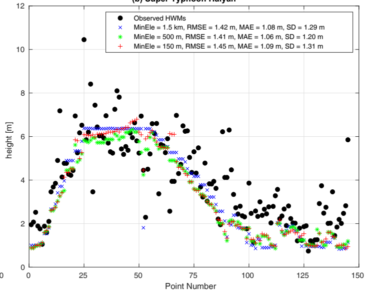
(b) Super Typhoon Haiyan
