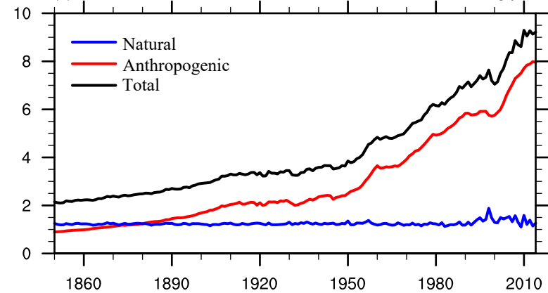
(c) BC emission
