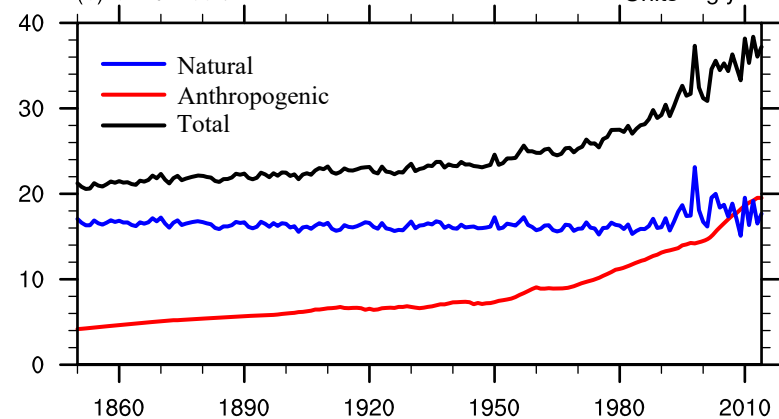
(b) OC emission
