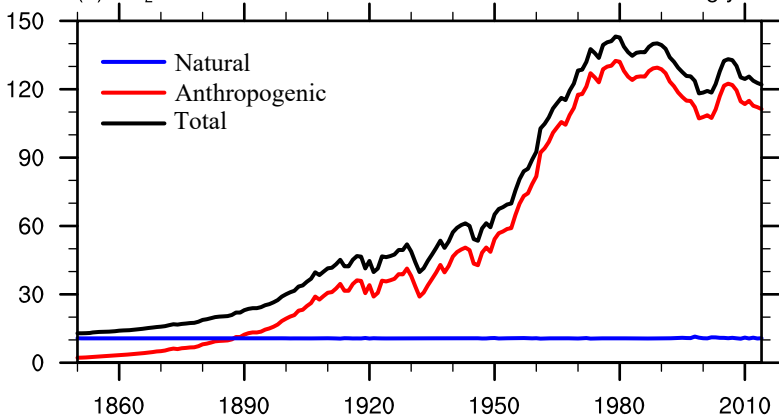
(a) SO 2 emission
