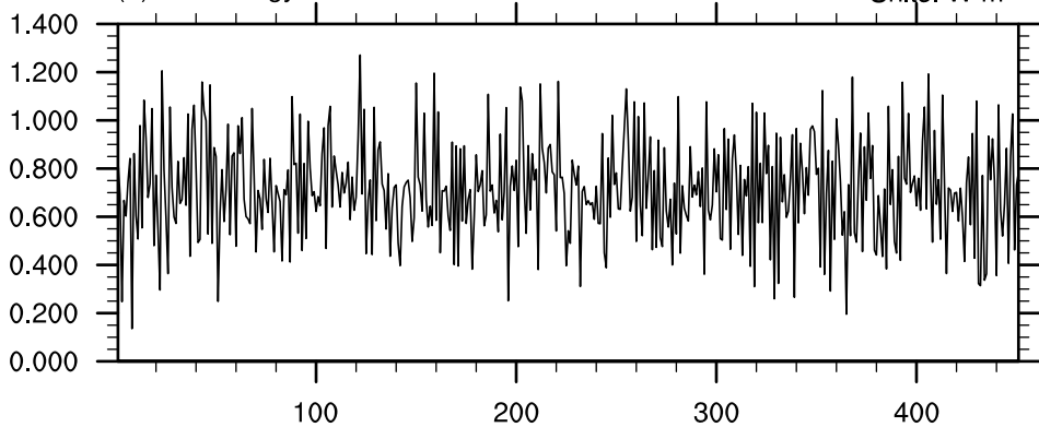
(a) Net energy at TOA
