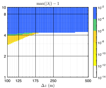
(b) ARK2(2,3,2)(1)
