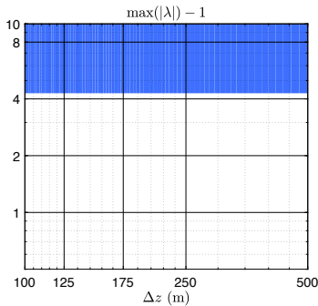
(c) ARK2(2,3,2)(2)
