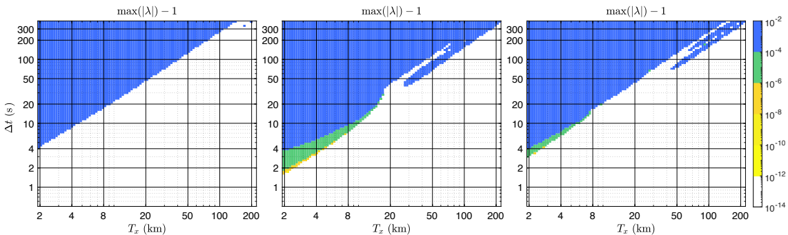
(a) Stability diagram for M2be
