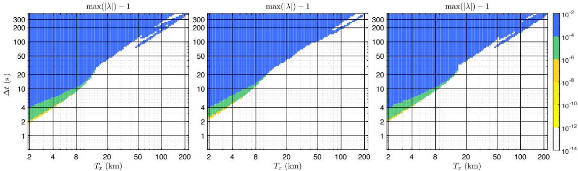
(a) Stability diagram for M2a
