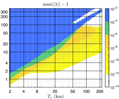
(c) System of normal modes, (T_x, \Delta t) axes
