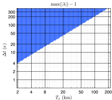
(b) 2-D acoustics system, (T_x, \Delta t) axes
