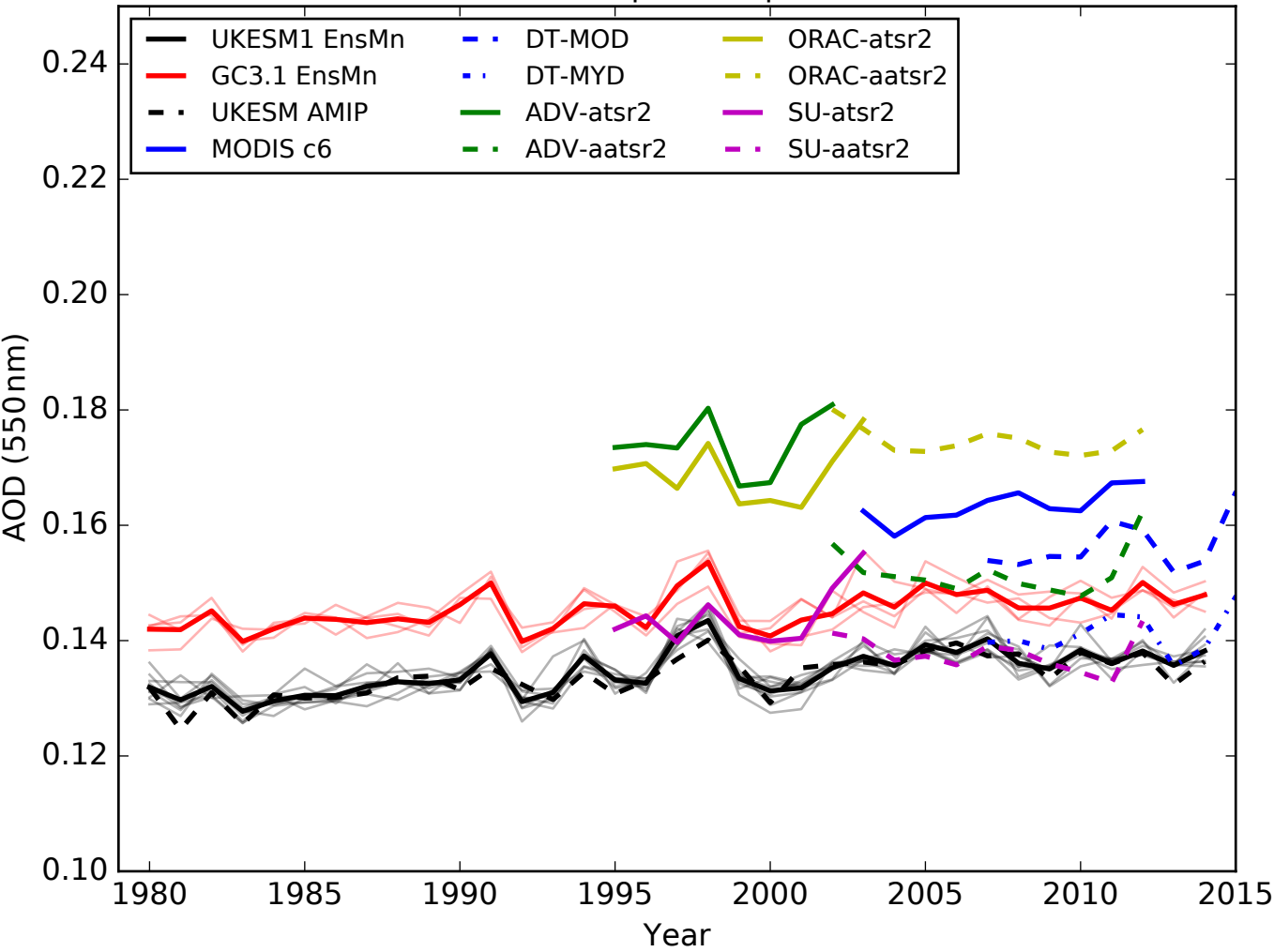
Total Aerosol Optical Depth (550 nm)
