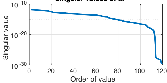
(c) Singular values of M
