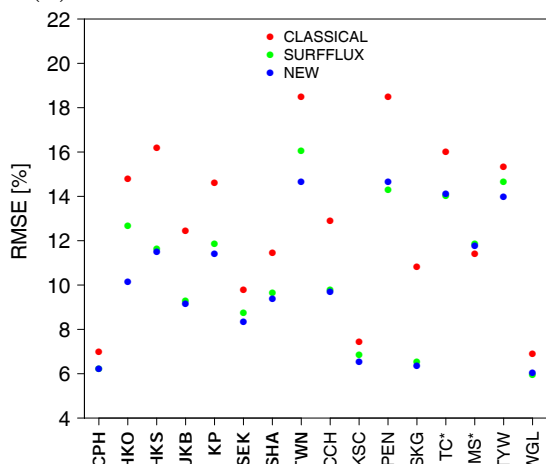
(f) Wind speed, RMSE
