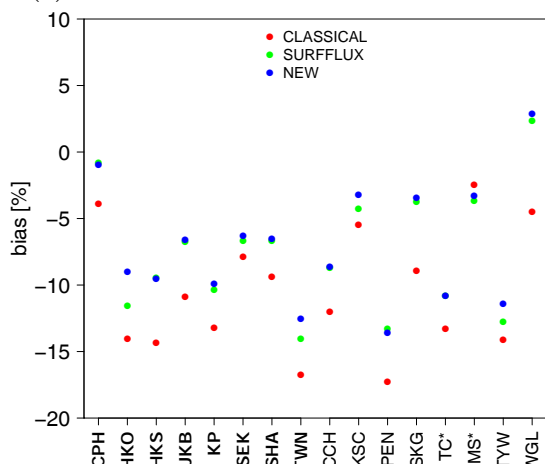
(e) Wind speed, bias
