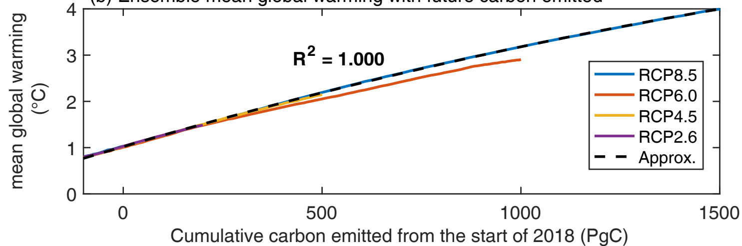
(b) Ensemble mean global warming with future carbon emitted
