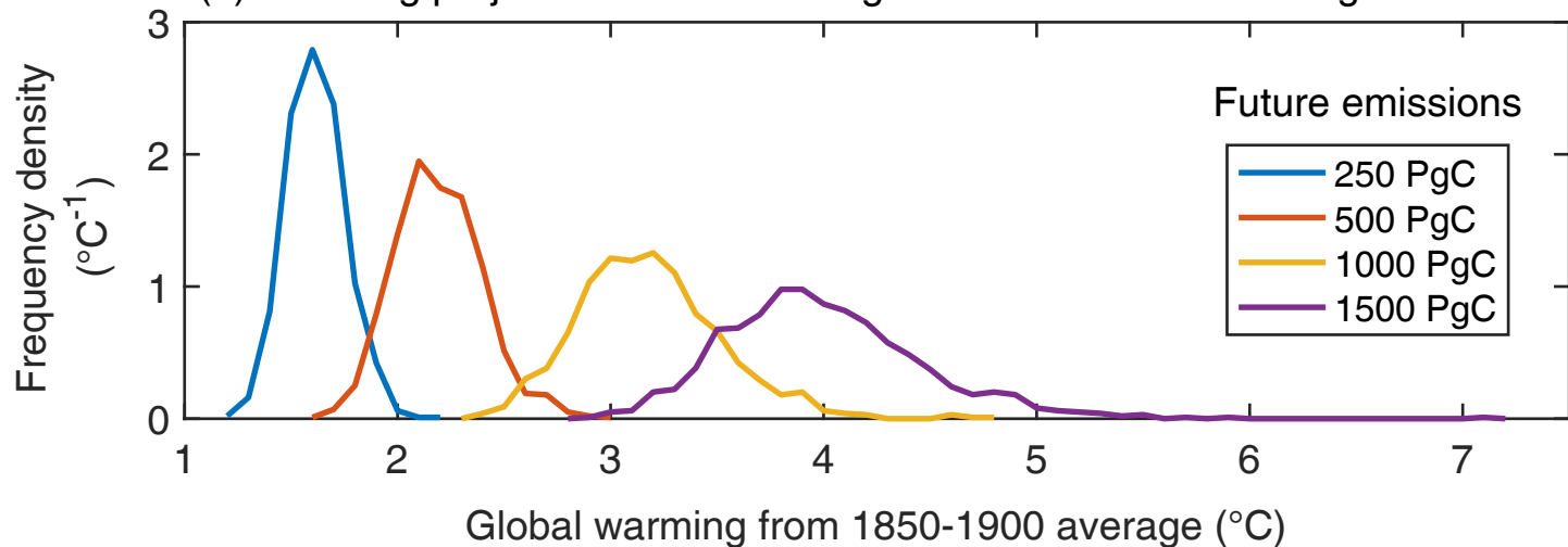
(b) Ensemble mean global warming with future carbon emitted
