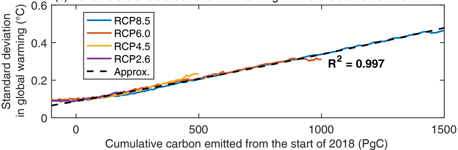
(c) Ensemble standard deviation in warming with future carbon emitted
