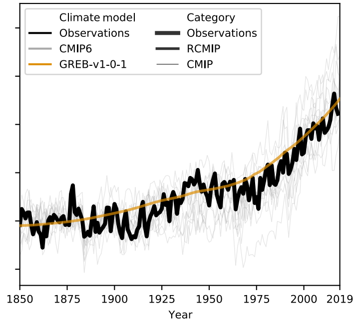
CO 2 -only effective radiative forcing
