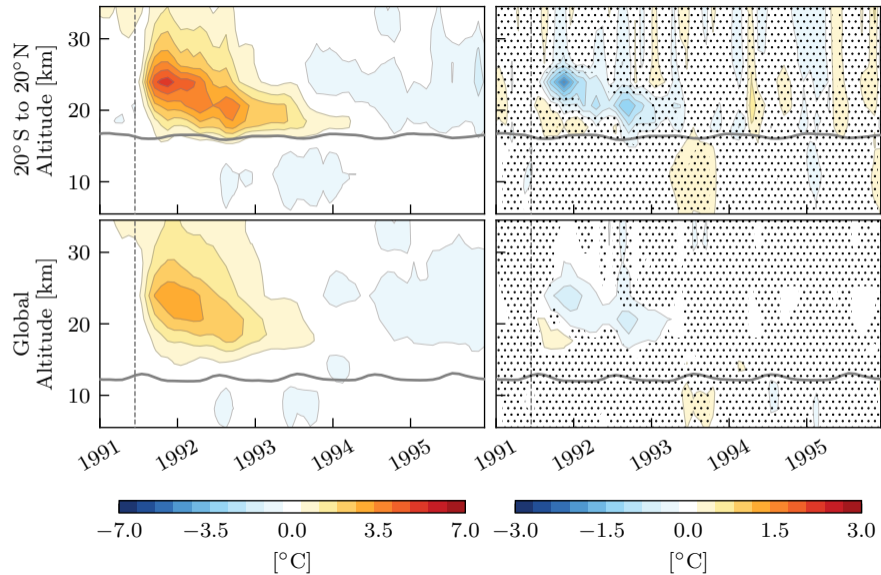
Temperature anomaly (v3)
