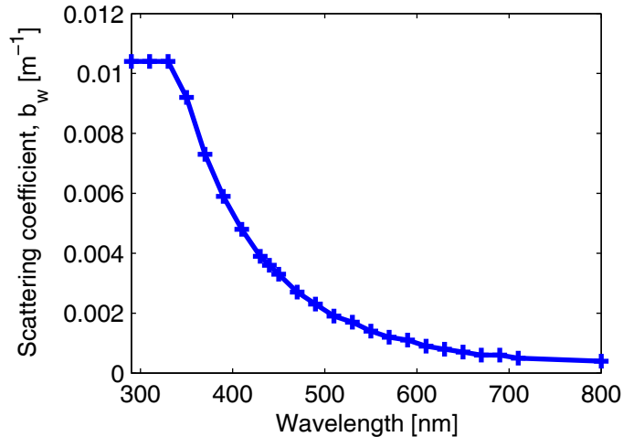
(c) Clear-water scattering
