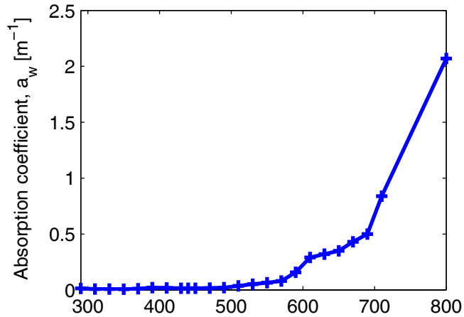
(b) Clear-water absorption
