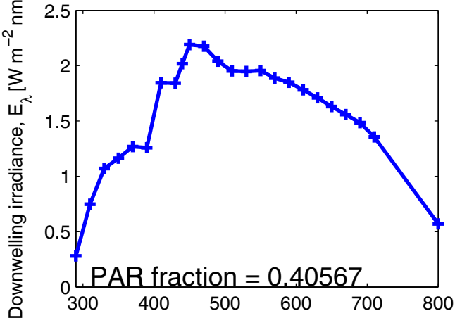
(a) Clear-sky energy spectrum
