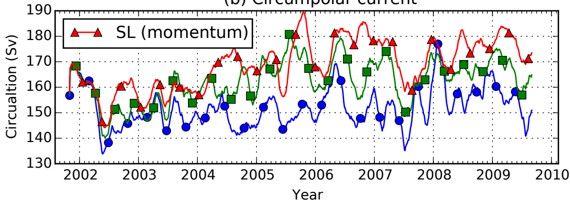
(b) Circumpolar current
