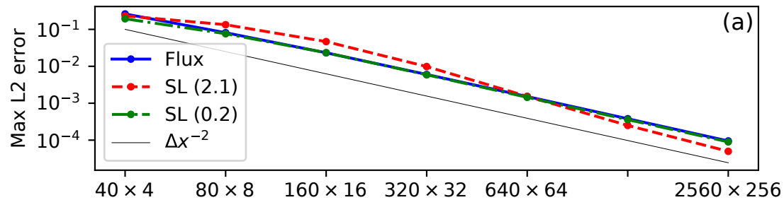
Convergence rate
