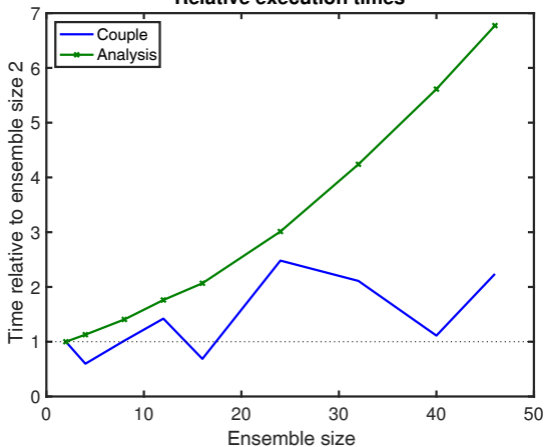
Relative execution times
