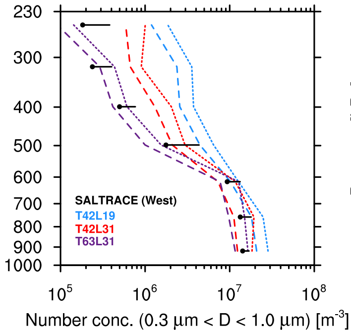
(a) SALTRACE (aircraft) vs. EMAC (MADE3)
