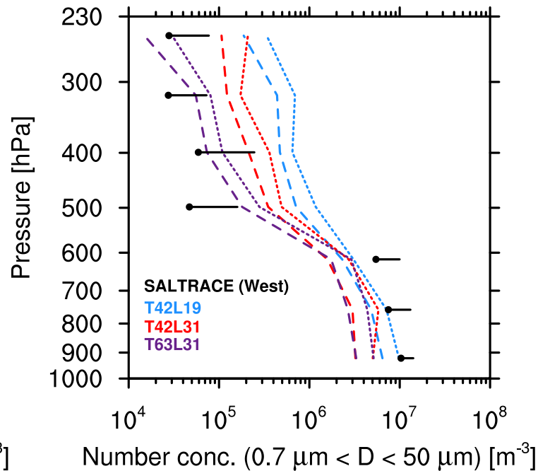
(b) SALTRACE (aircraft) vs. EMAC (MADE3)
