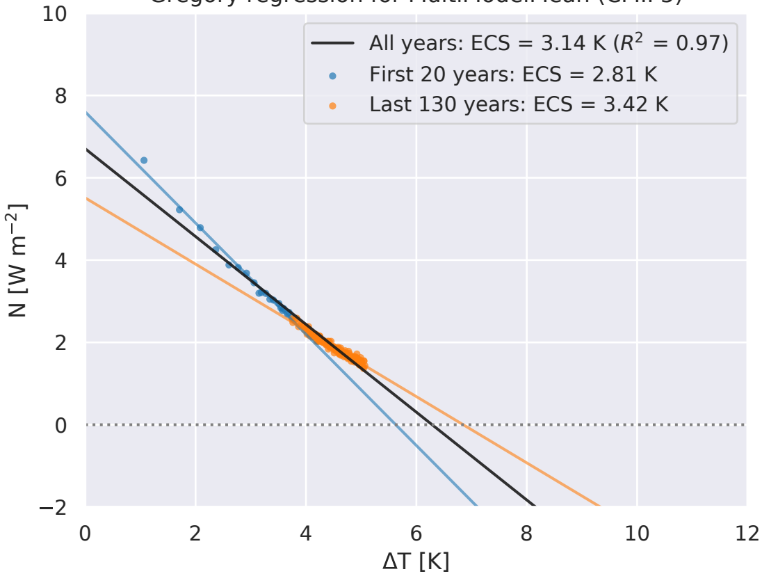
Gregory regression for MultiModelMean (CMIP5)
