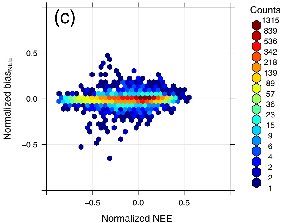
Bias NEE from linear LSWI prediction
