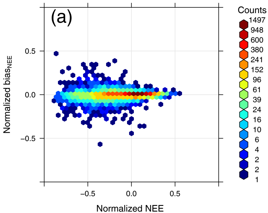
Bias NEE from linear EVI prediction
