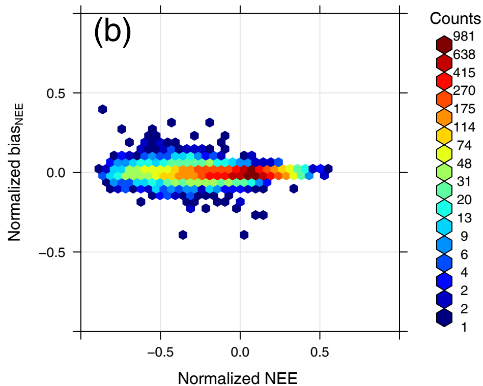
Bias NEE from persistence EVI prediction
