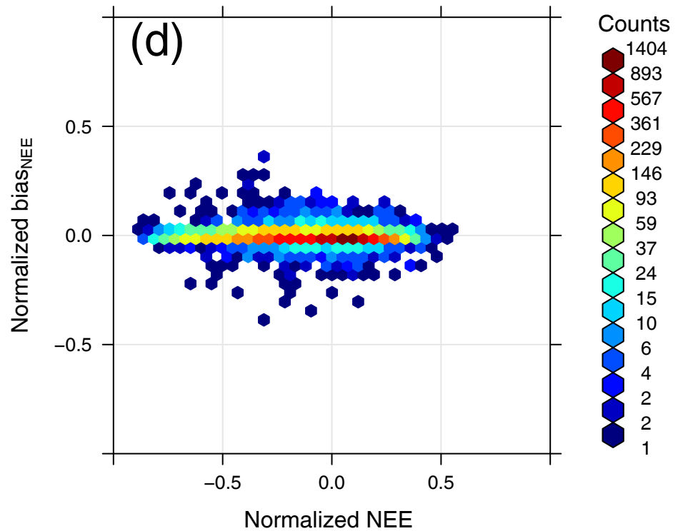
Bias NEE from persistence LSWI prediction
