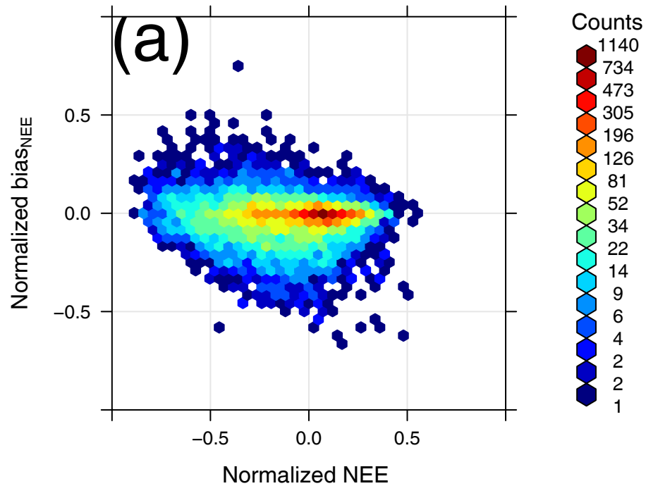
Bias NEE from SW forecasting
