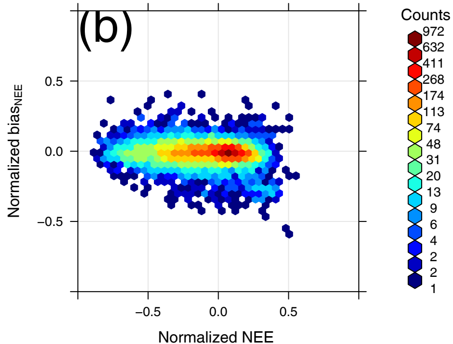
Bias NEE from temperature forecasting
