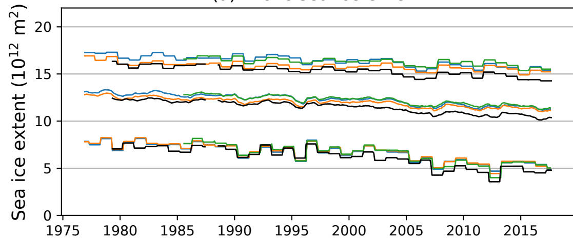
(a) Arctic sea ice extent
