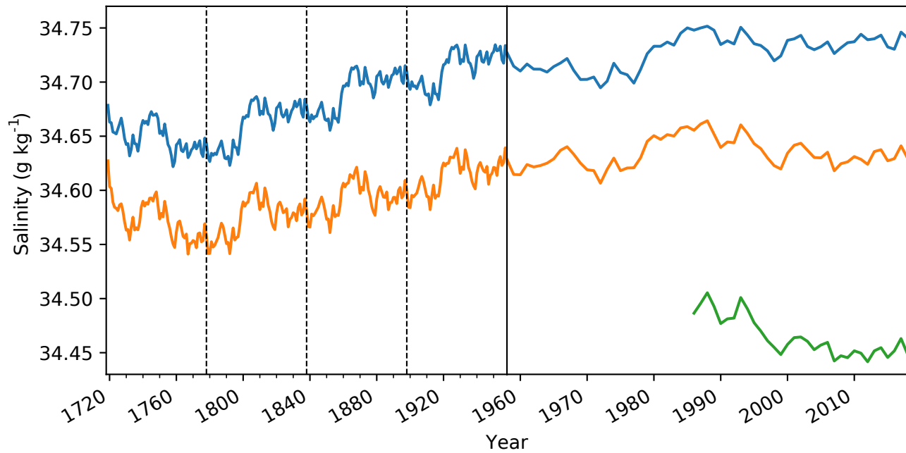
(c) Global average surface salinity
