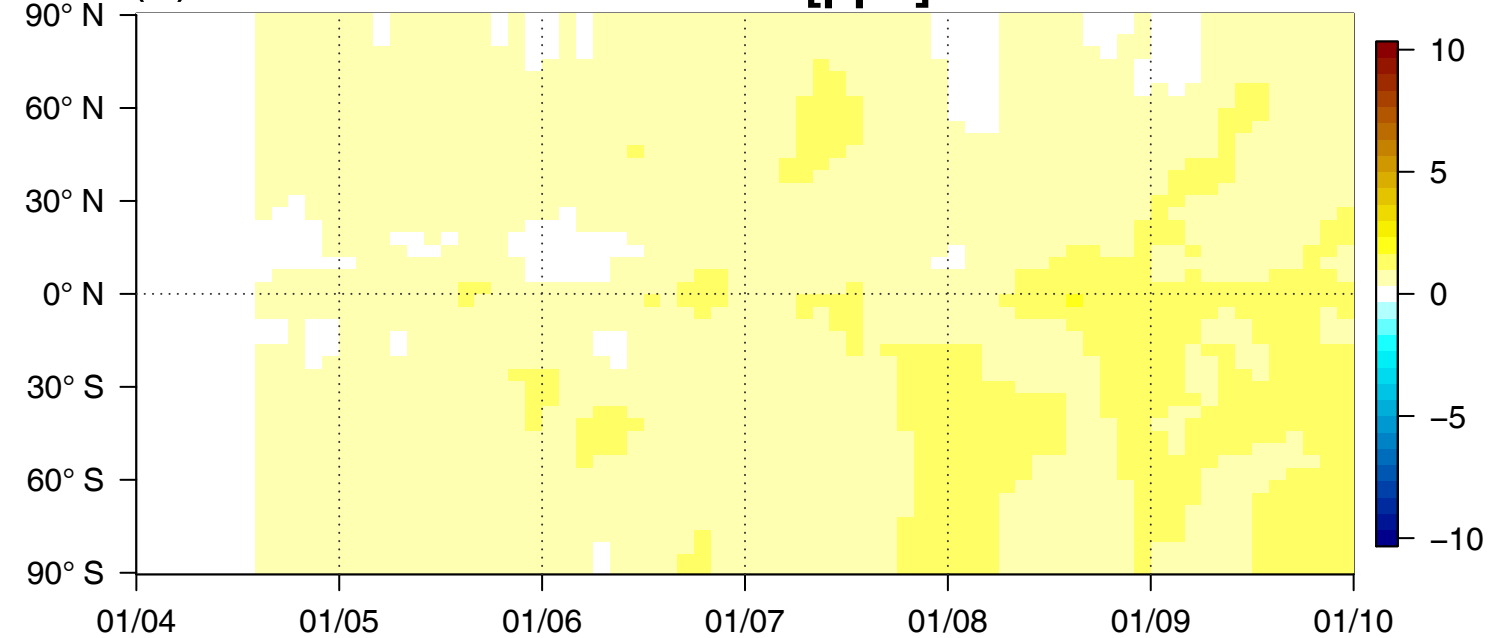
Mean zonal dXCH 4 time series
