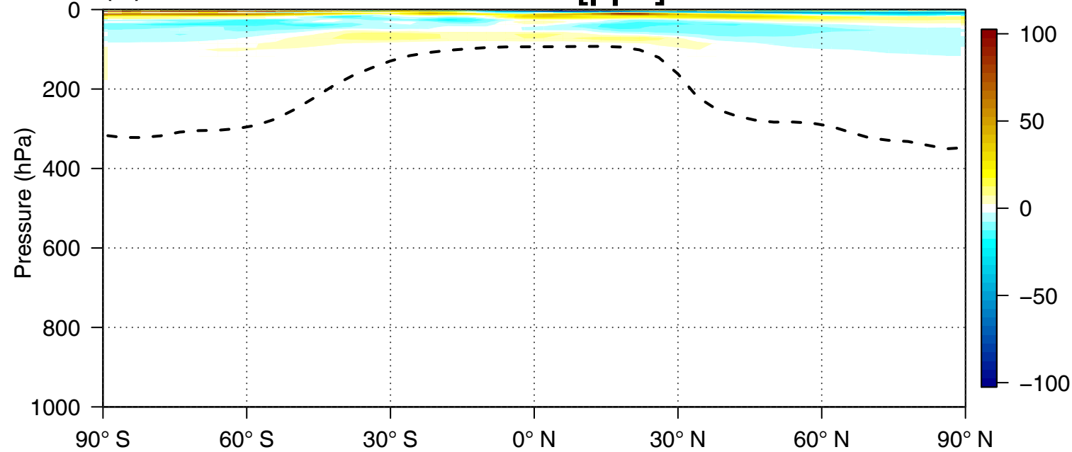
Mean zonal dCH 4 on 2010/01 after 6 years spin up
