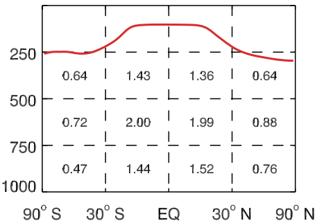
(c) Spivakovsky et al. (2000) climatology OH burden
