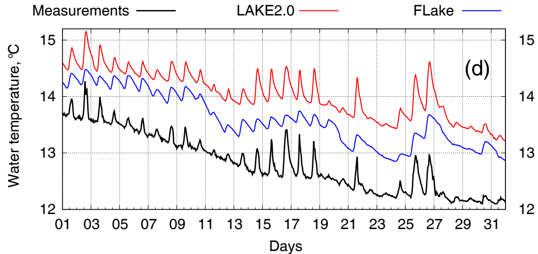
Mixed layer water temperature, January 2019
