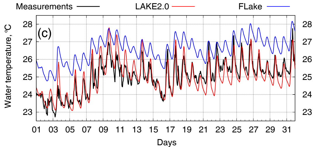
Mixed layer water temperature, July 2018
