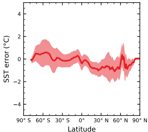
(c) Zonal mean SST error CMIP5
