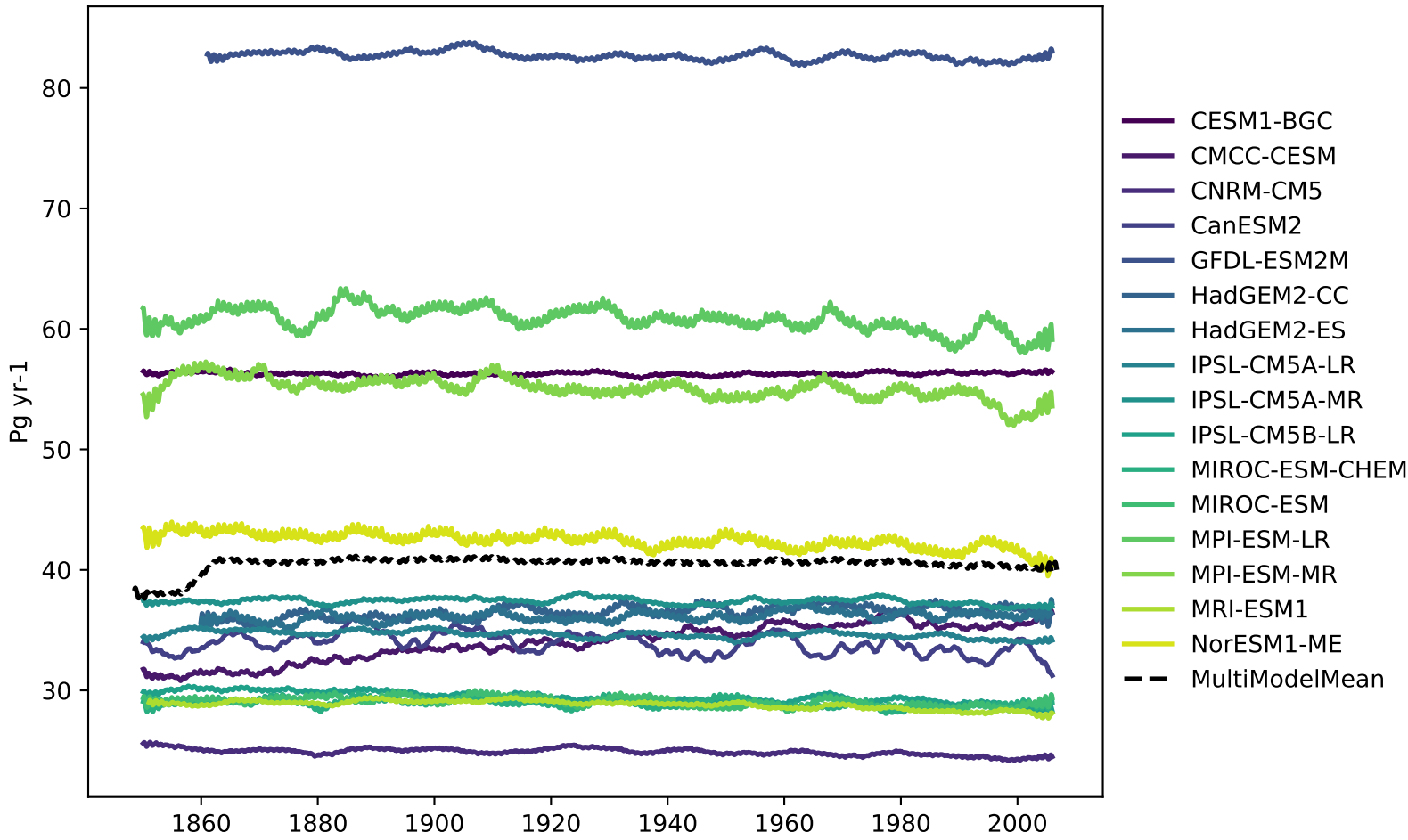
Global total primary organic carbon production by all types of phytoplankton
