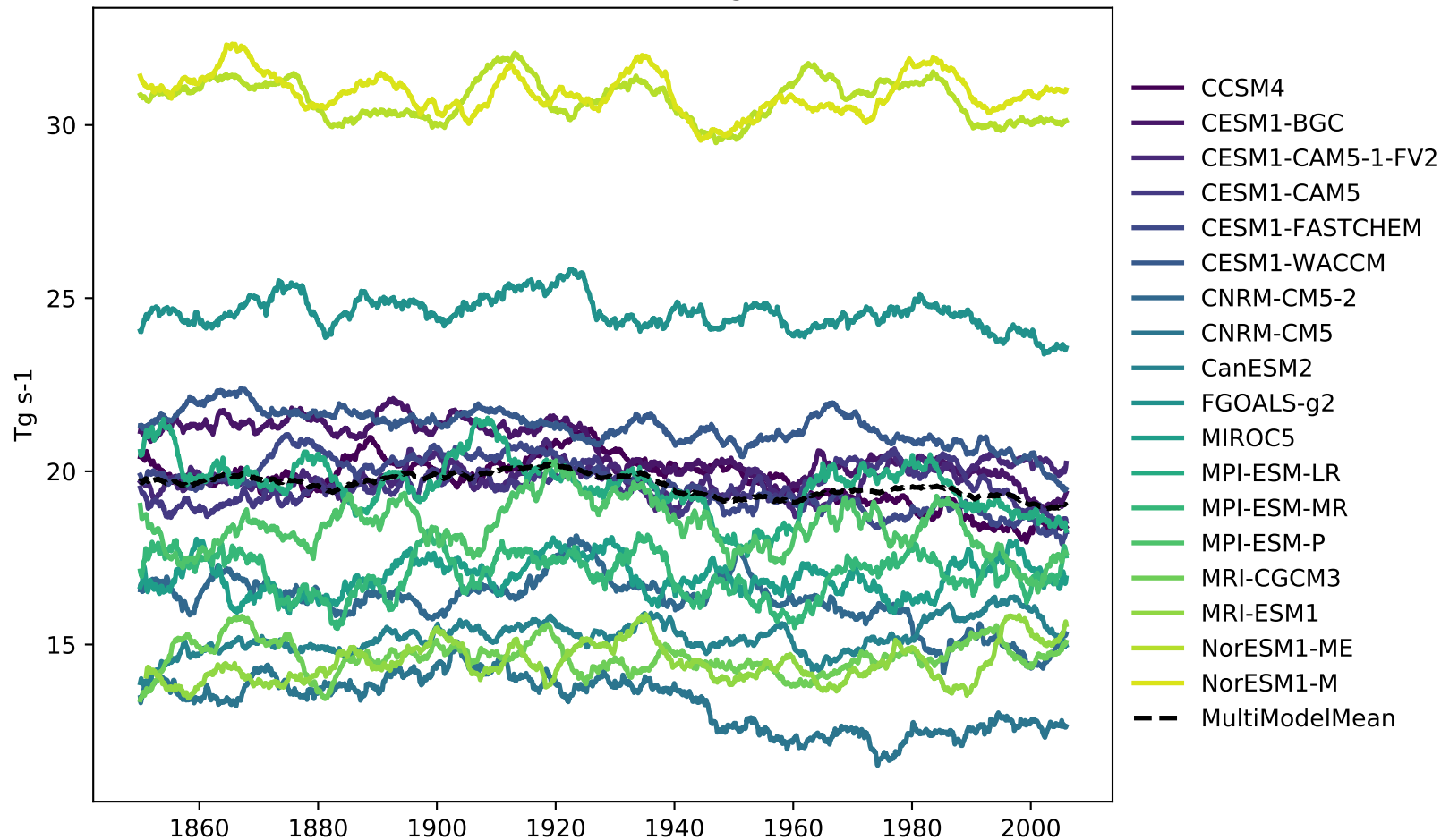
Atlantic Meridional Overturning Circulation
