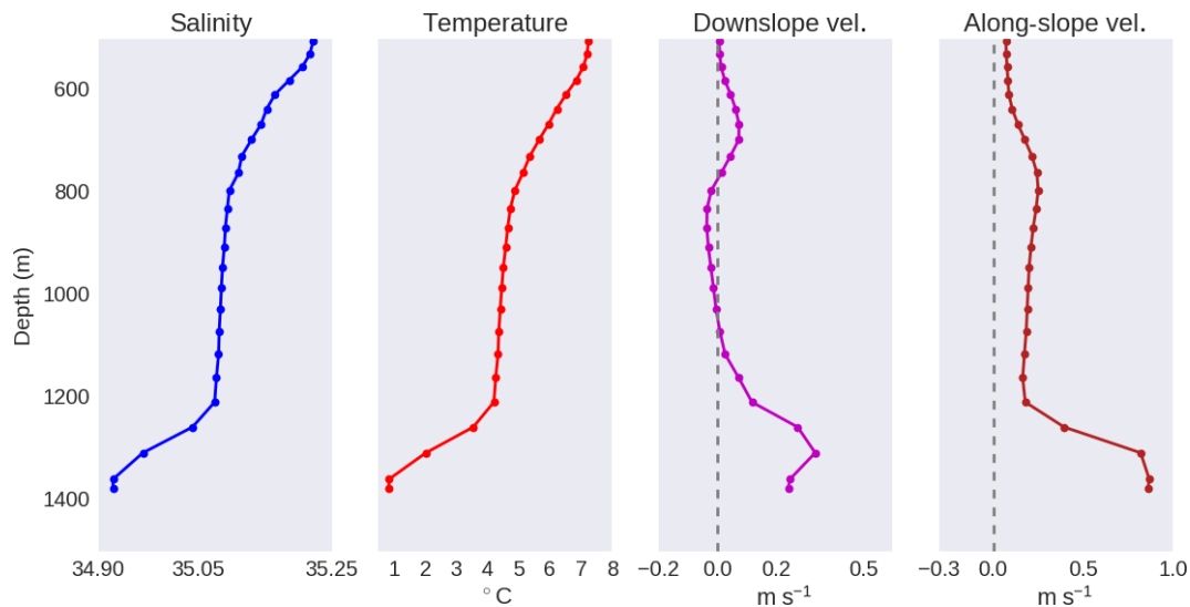
Figure 15. Vertical profiles of the physical properties of the overflow plume in simulation DSO60.L150 (hour 10 on 1 February of year 5) at section 16 for the location indicated with a white-rimmed dot in Fig. 6b. (a) Salinity, (b) temperature, (c) cross-slope velocity, and (d) along-slope velocity.
