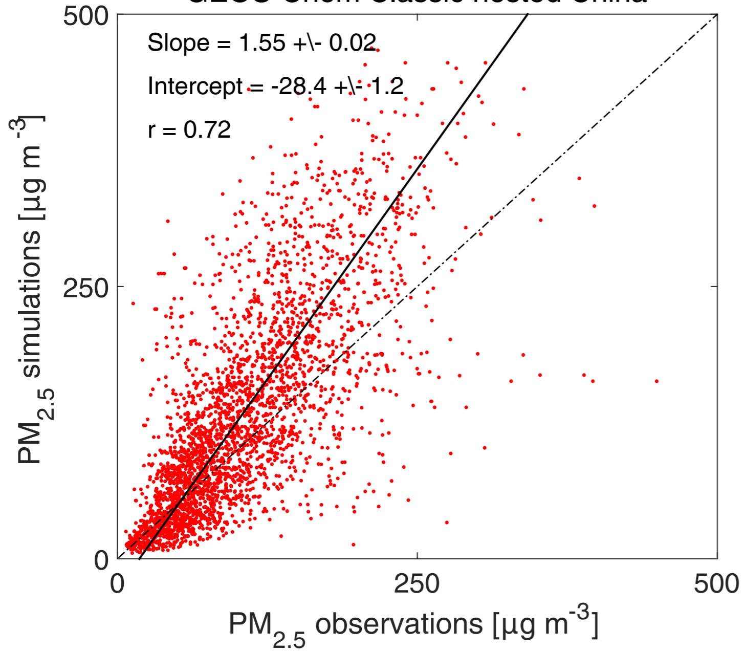
GEOS-Chem Classic nested China
