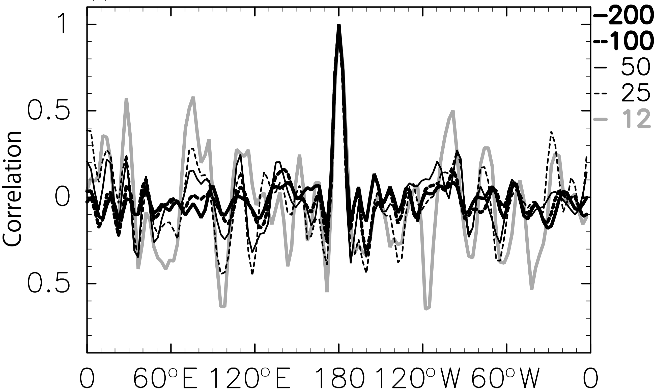
(a) 10 hPa
