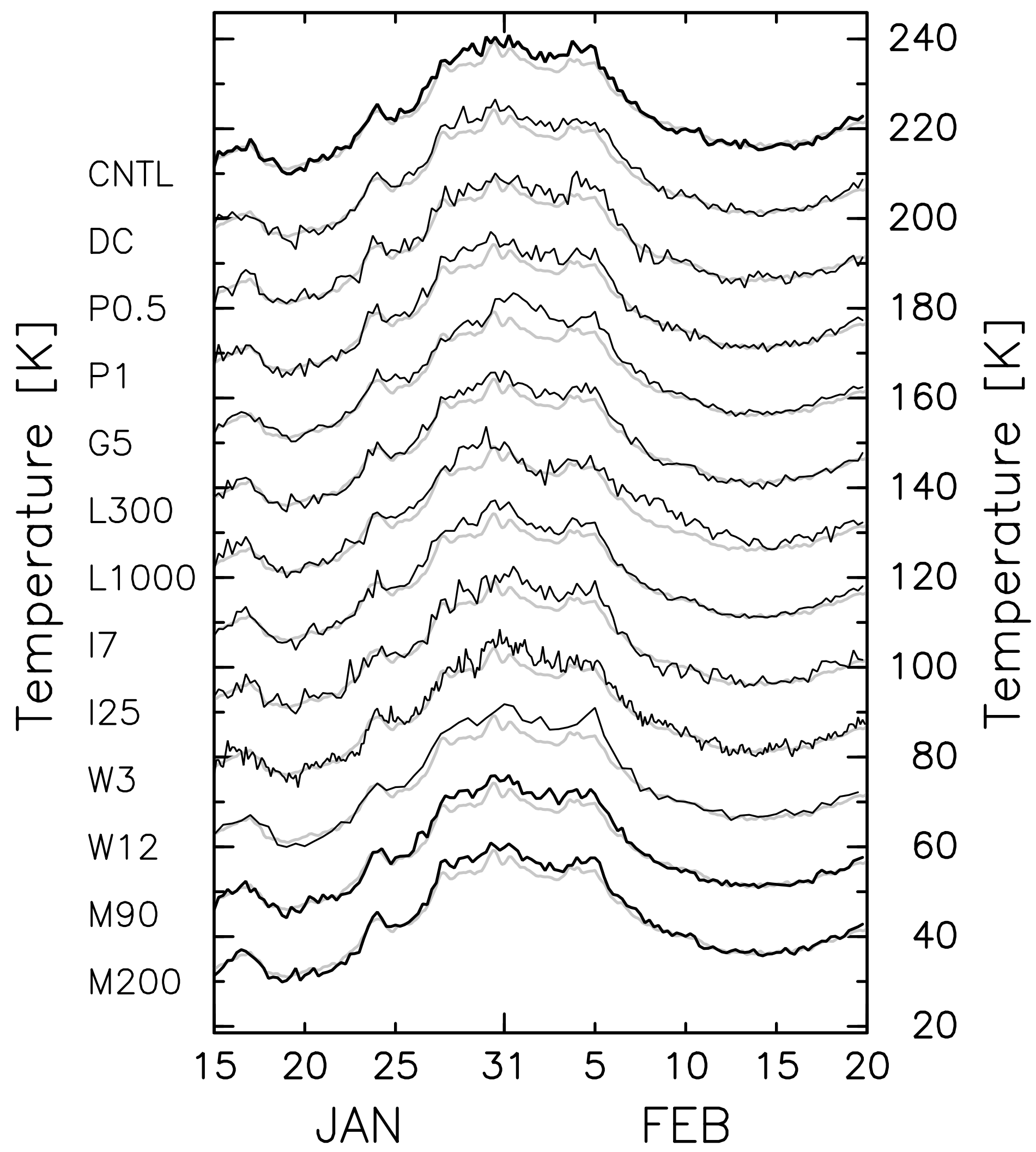
(b) T 10.0 hPa 70° N
