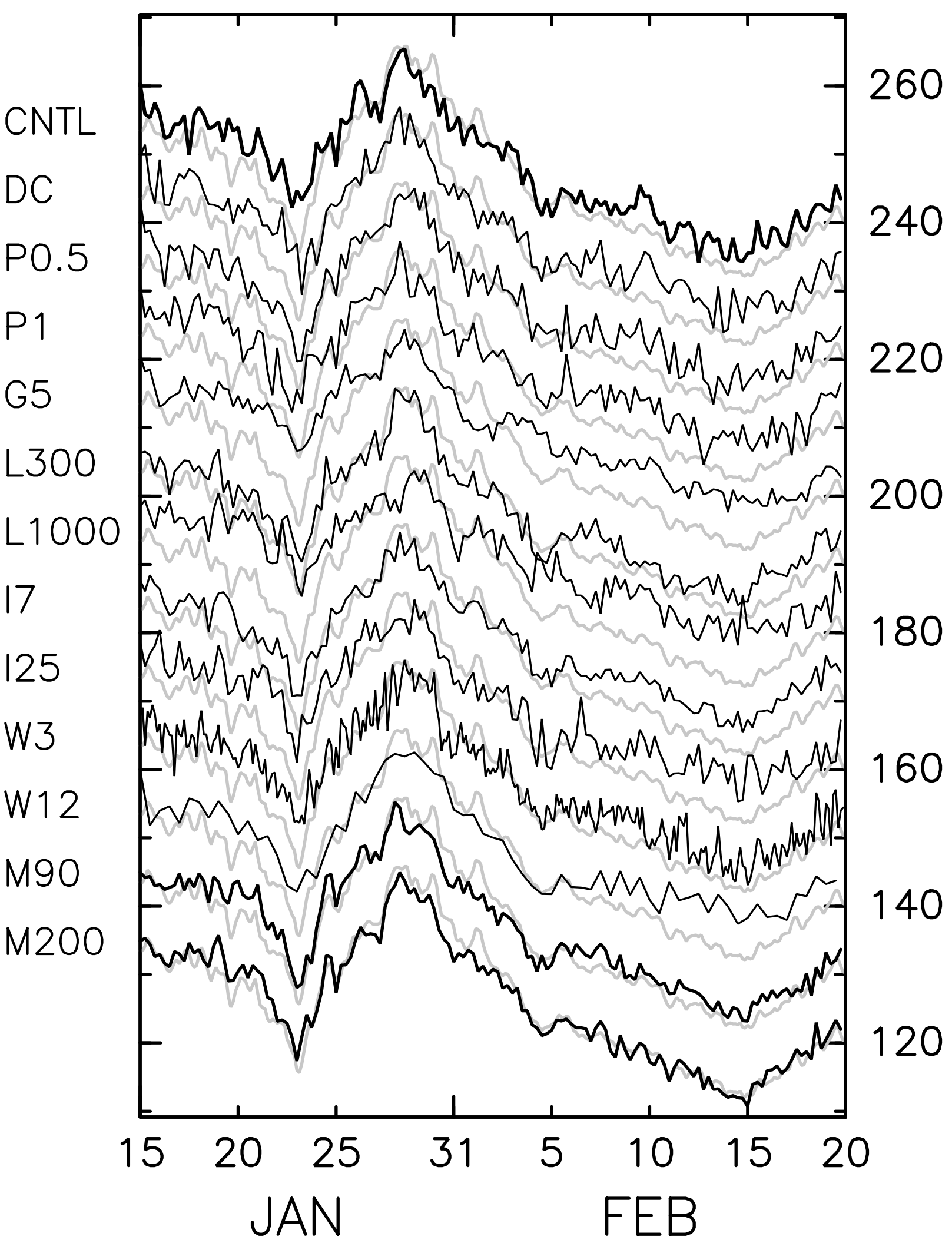
(c) T 1.0 hPa 70° N
