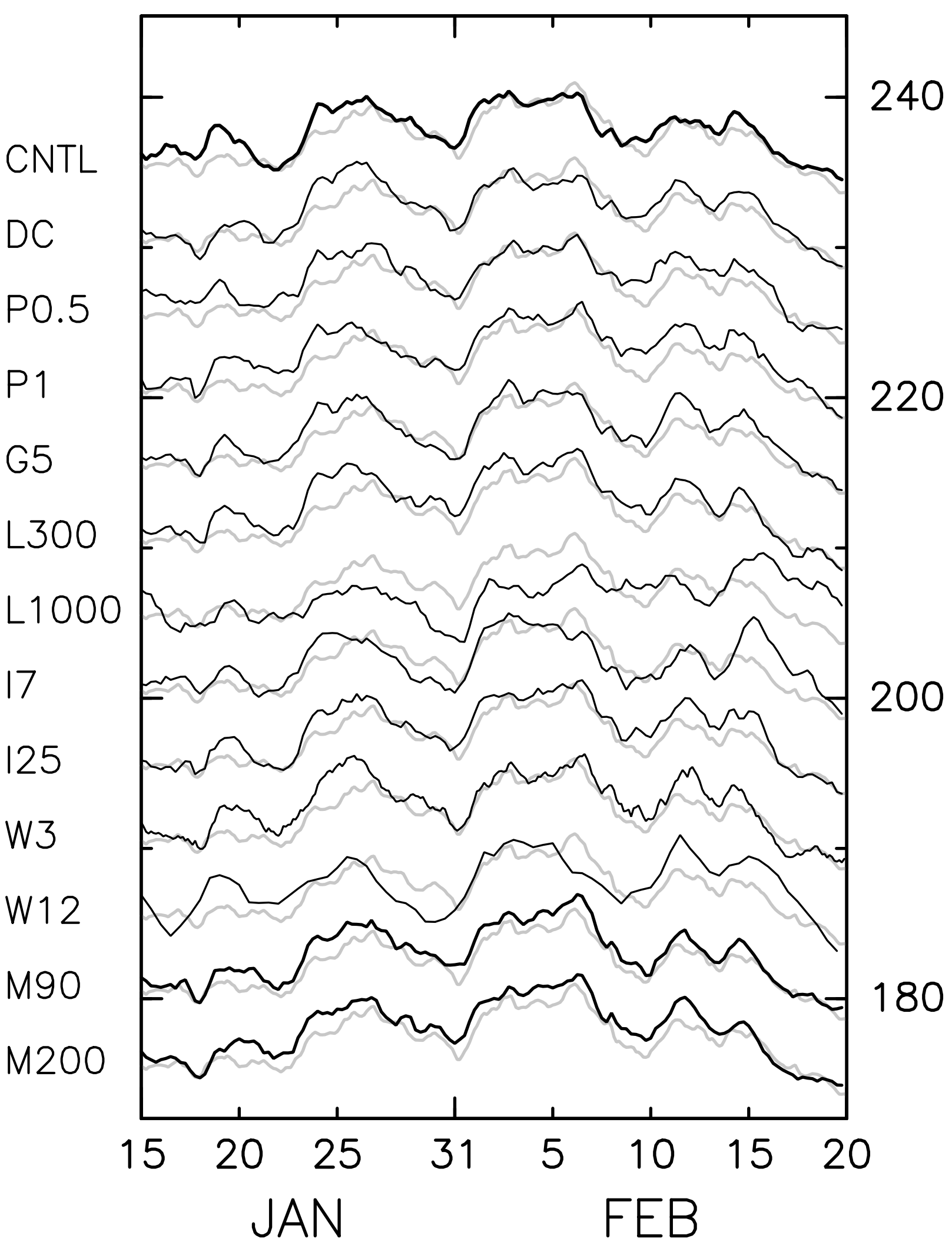
(a) T 500.0 hPa 70° N
