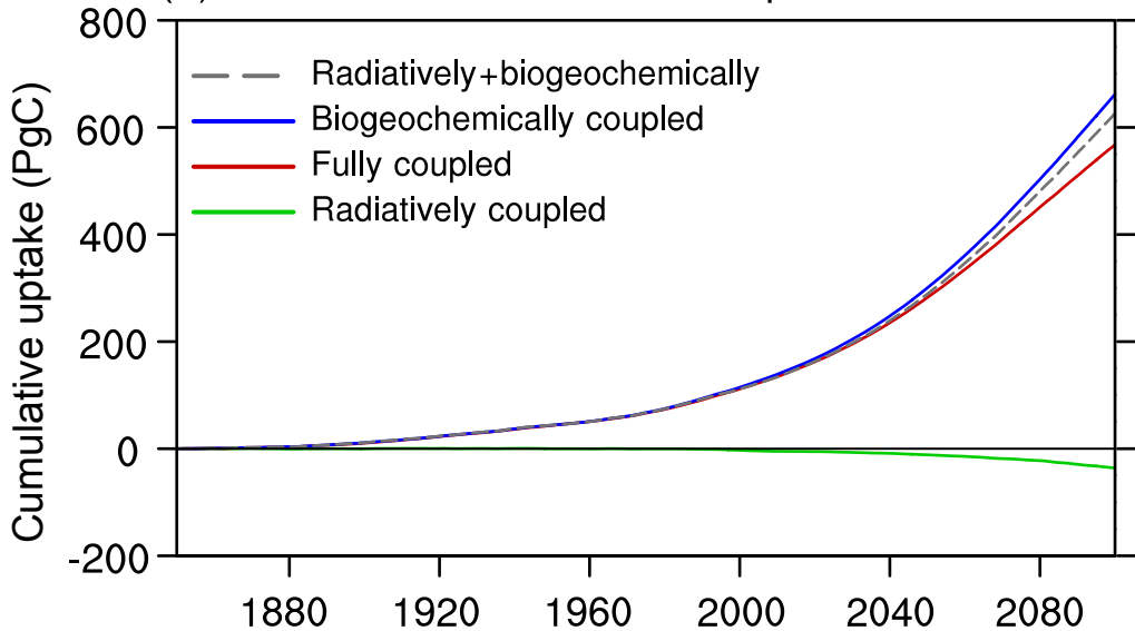
(b) Cumulative oceanic carbon uptake
