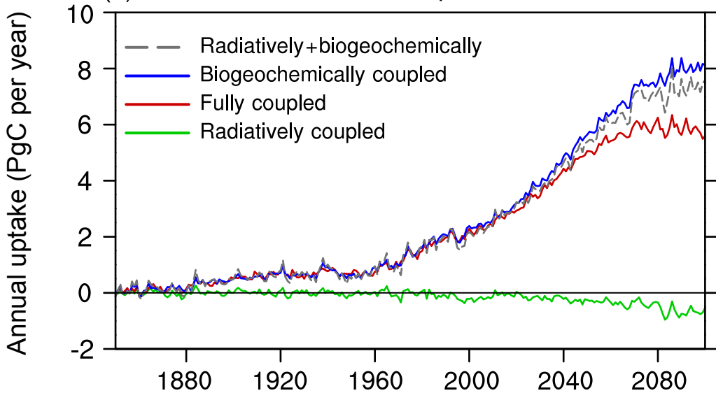
(a) Annual oceanic carbon uptake
